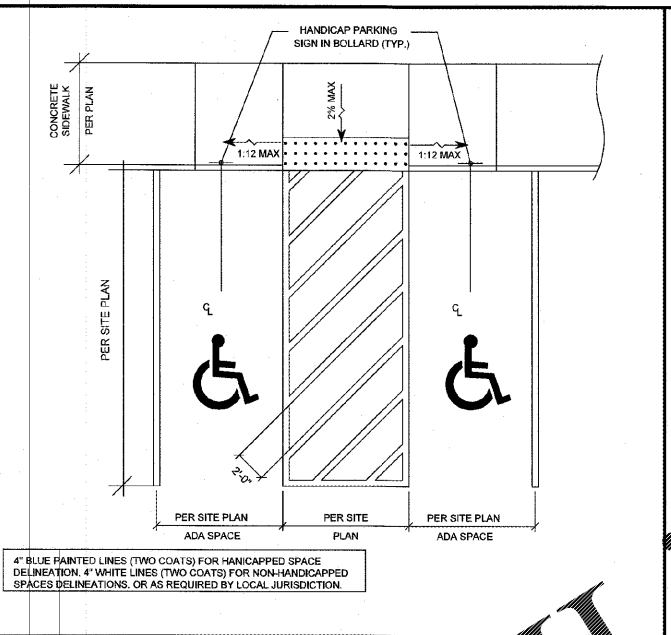
ADA PARKING LAYOUT DETAIL NOT TO SCALE
