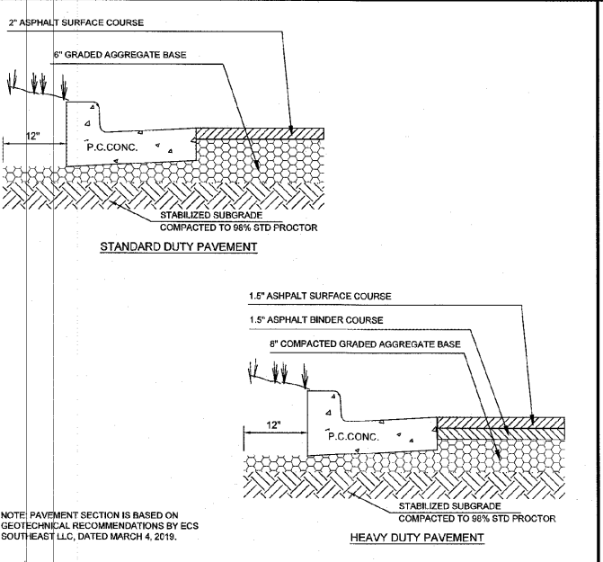
PAVEMENT SECTION DETAIL NOT TO SCALE
