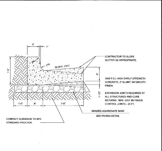
CURB & GUTTER DETAIL NOT TO SCALE
