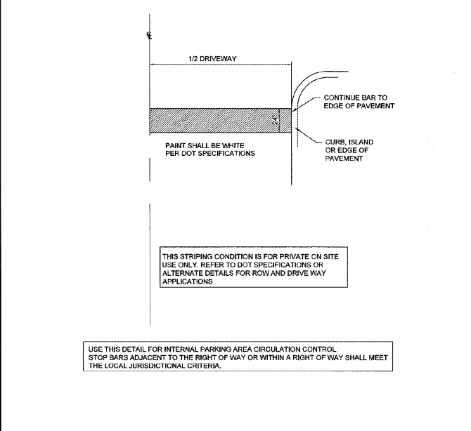
STOP BAR DETAIL NOT TO SCALE
