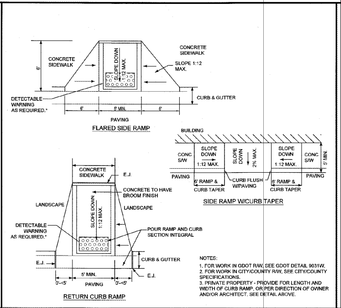
ADA PARKING RAMP DETAIL NOT TO SCALE
