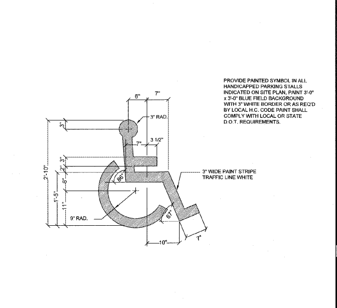
ADA PARKING SYMBOL DETAIL NOT TO SCALE
