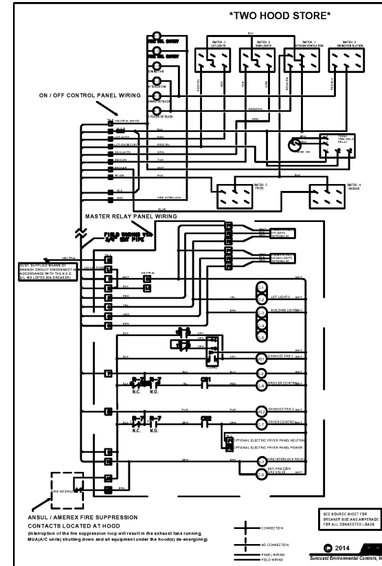
PANEL SCHEMATIC DIAGRAMS
