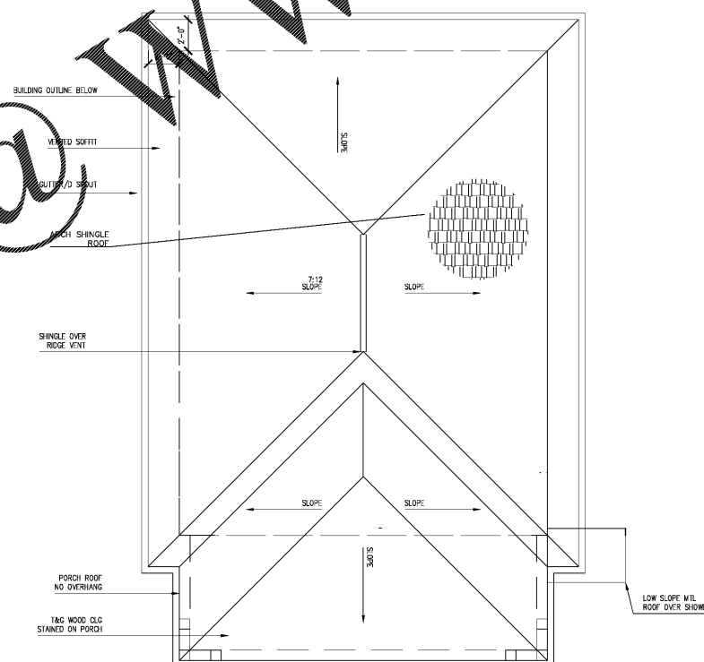
1 ROOF PLAN SCALE: 1/4"=1'-0"
