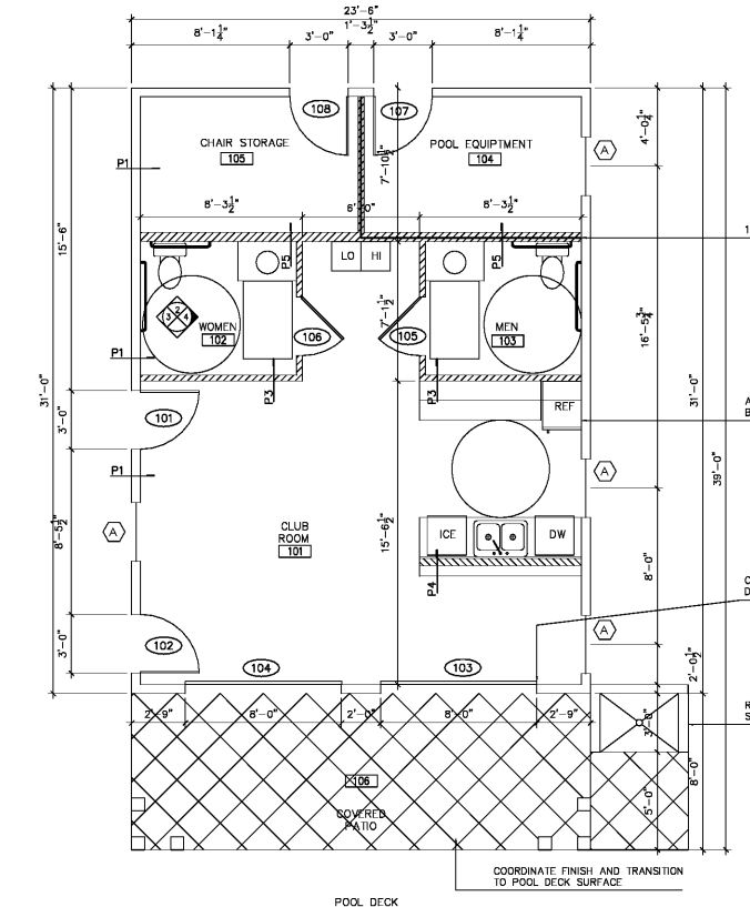
1 FLOOR PLAN SCALE: 1/4" = 1'-0"
