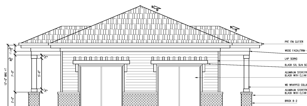
1 ELEVATION - FRONT SCALE: 1/4"=1'-0"
