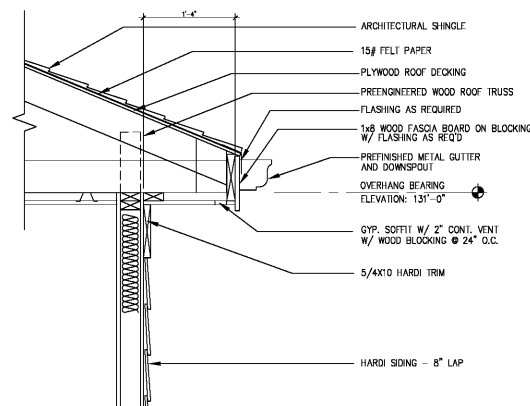
3 DETAIL: Roof Overhang SCALE: 1"=1'-0"
