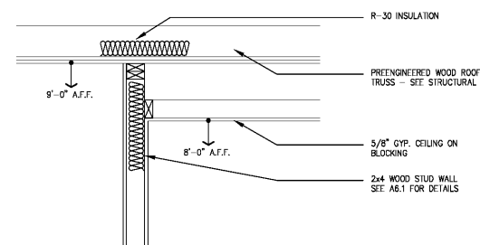
4 DETAIL: Gyp. Ceiling SCALE: 1"=1'-0"
