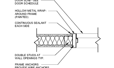
3 TYP. INTERIOR JAMB DETAIL 1 1/2" = 1'-0"
