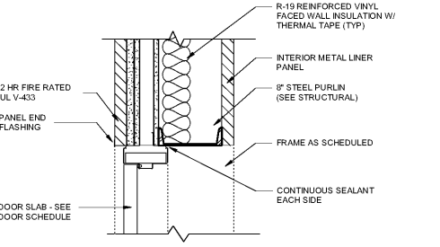
4 TYP. HEAD/JAMB @ 2 HR WALL 1 1/2" = 1'-0"
