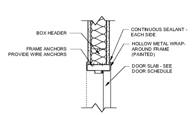
2 TYP. INTERIOR HEAD DETAIL 1 1/2" = 1'-0"
