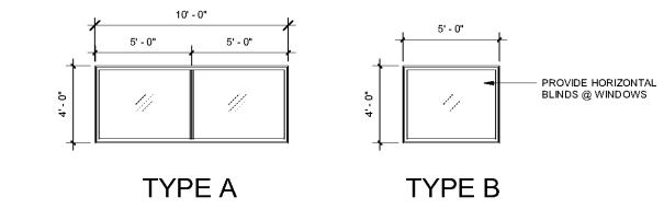
WINDOW SCHEDULE 1/4" = 1'-0"
