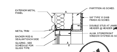
12 INTERIOR STOREFRONT HEAD/JAMB DETAIL 1 1/2" = 1'-0"
