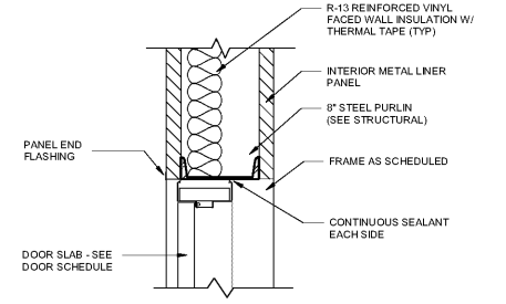
5 TYP. HEAD/JAMB @ EXT. WALL 1 1/2" = 1'-0"
