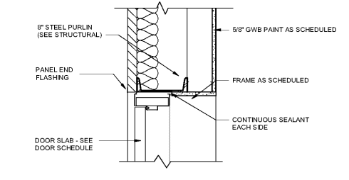
9 TYP. HEAD/JAMB @ EXT. WALL@OFFICE 1 1/2" = 1'-0"
