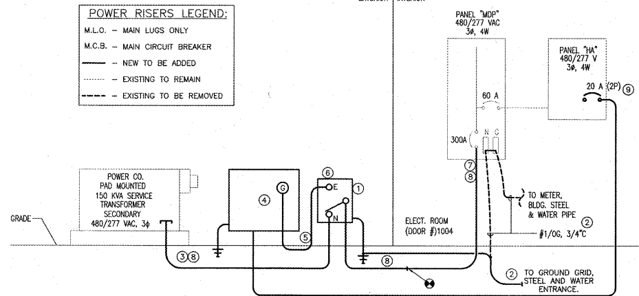
01 HANGER #2 POWER RISER E-2 NO SCALE
