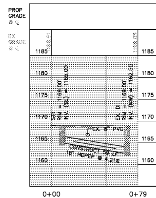
ST1 TO EX. DI. PROFILE VIEW HORIZONTAL SCALE: 1"=40' VERTICAL SCALE: 1"=10'
