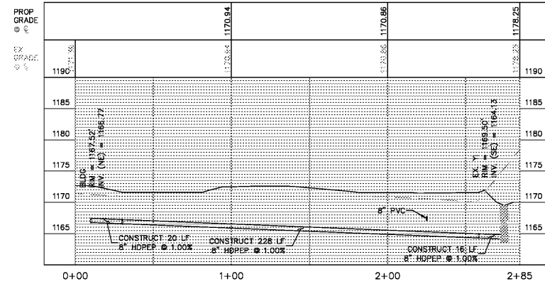
ROOF DRAIN TO EX. DI. PROFILE VIEW HORIZONTAL SCALE: 1"=40' VERTICAL SCALE: 1"=10'
