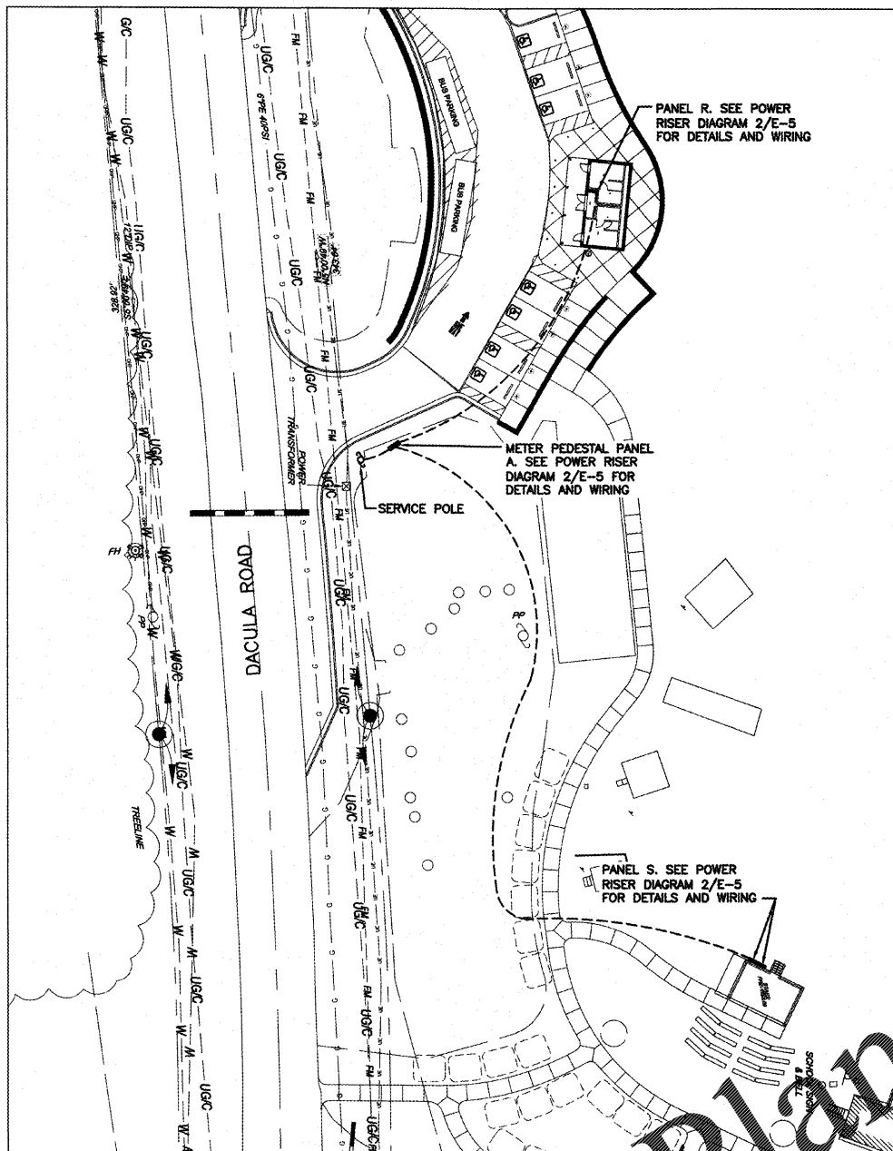
1 OVERALL SITE PLAN - POWER E-5 SCALE: 1" = 30'-0"
