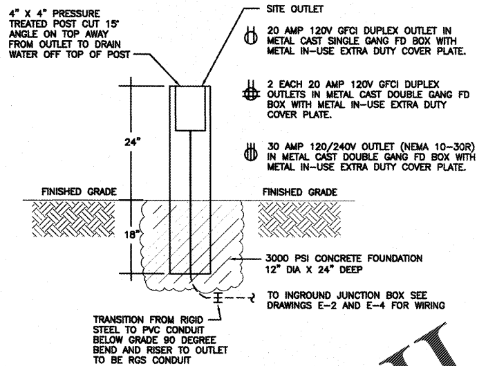
3 SITE OUTLET MOUNTING DETAIL E-5 SCALE: NTS
