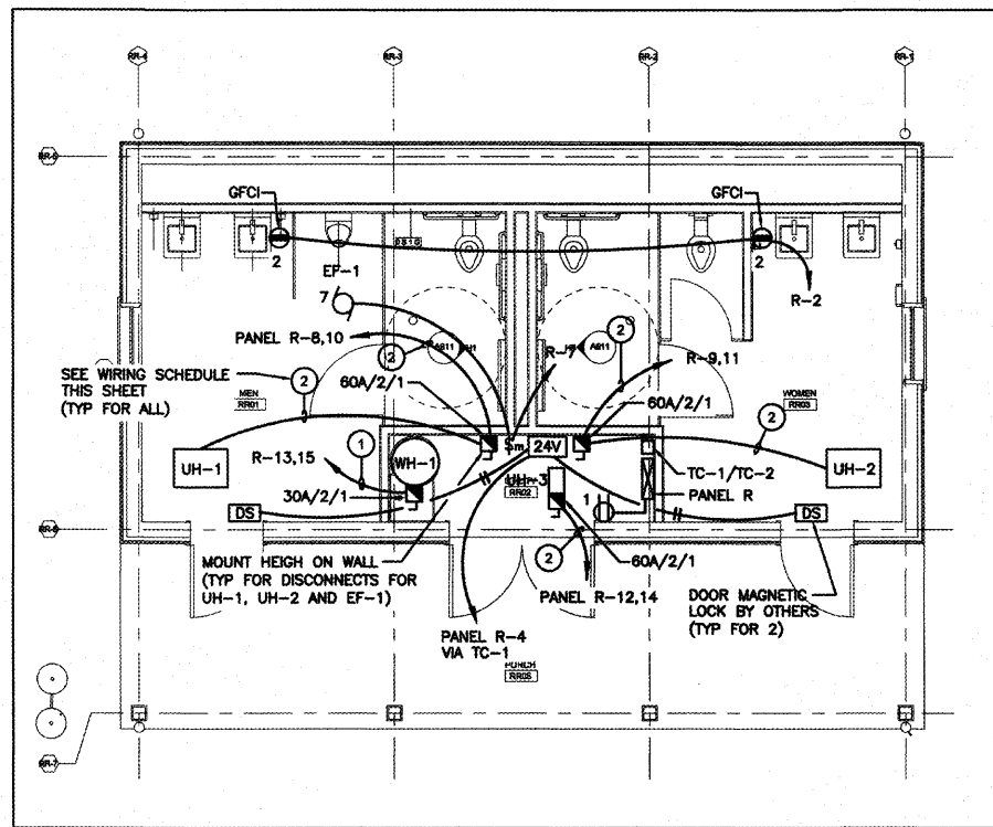
1 FLOOR PLAN - POWER E-3 SCALE: 1/4" = 1'-0"
