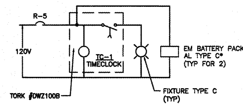
4 CONTROL SCHEMATIC E-3 SCALE: NTS
