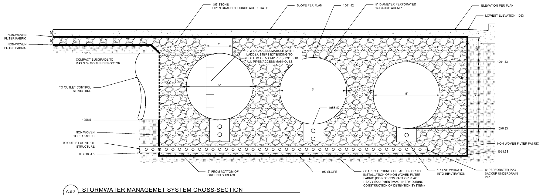
C-6.2 STORMWATER MANAGEMENT SYSTEM CROSS-SECTION
