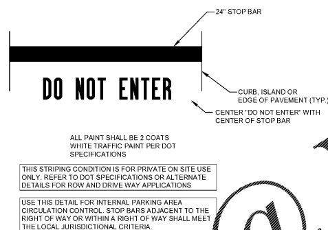
C-6 "DO NOT ENTER" LABEL STRIPING NOT TO SCALE
