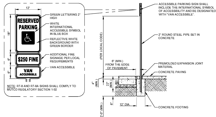
C-6 SIDEWALK POLE MOUNTED ACCESSIBLE SIGNAGE NOT TO SCALE
