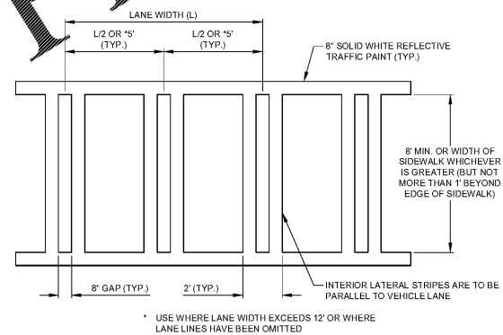
C-6 CROSSWALK STRIPING NOT TO SCALE
