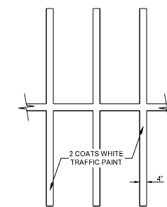
C-6 PAVEMENT STRIPING NOT TO SCALE
