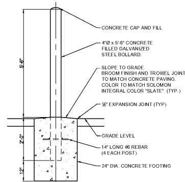
C-6 BOLLARD NOT TO SCALE
