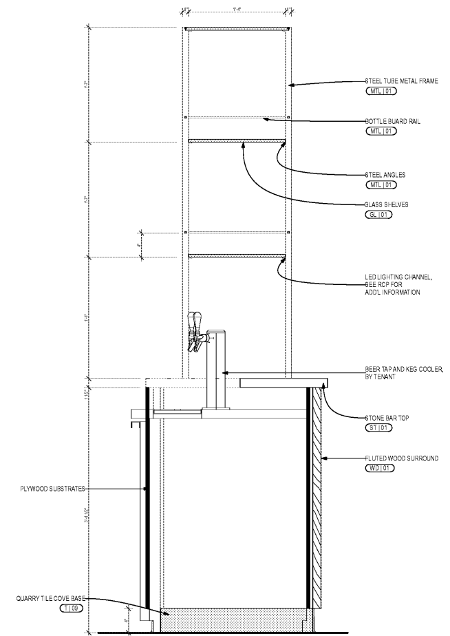
1 BAR ISLAND SECTION SCALE: 1 1/2\"/>
