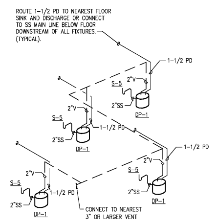
5 PUMP WASTE RISER DIAGRAM P5 SCALE: NTS
