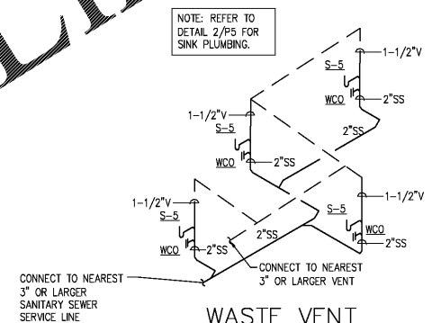
4 WASTE VENT RISER DIAGRAM P5 SCALE: NTS
