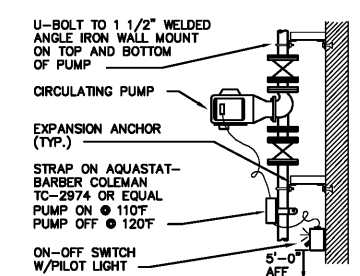
IN-LINE CIRCULATING PUMP WALL MOUNTING DETAIL NO SCALE
