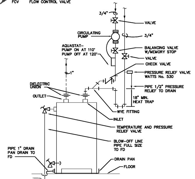
ELECTRIC WATER HEATER PIPING DIAGRAM NO SCALE
