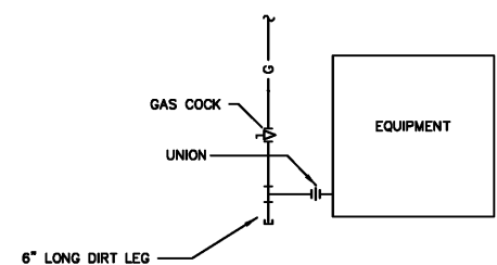
GAS CONNECTION TO EQUIPMENT SCALE: NONE
