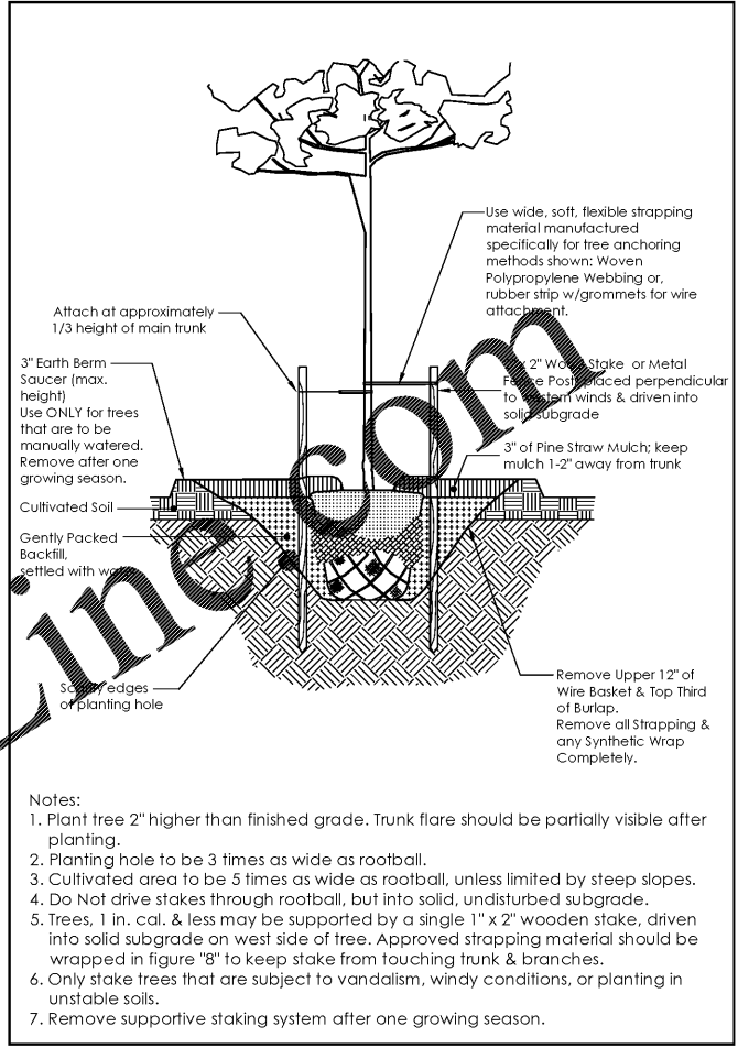
Tree Planting Detail & Small Tree (<= 2 in. cal.) Staking Detail (not to scale)
