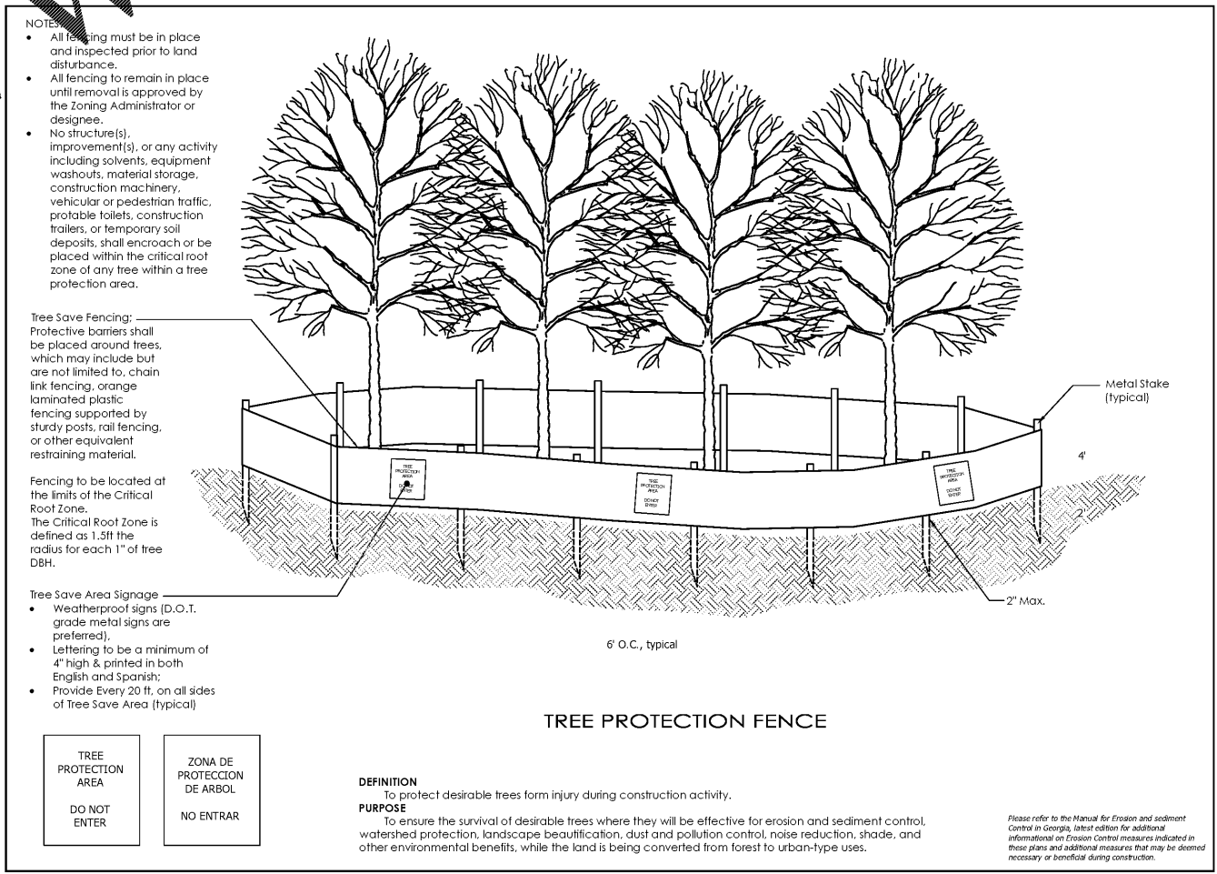
Tree Protection - Active Tree Protection Fence Detail (not to scale)
