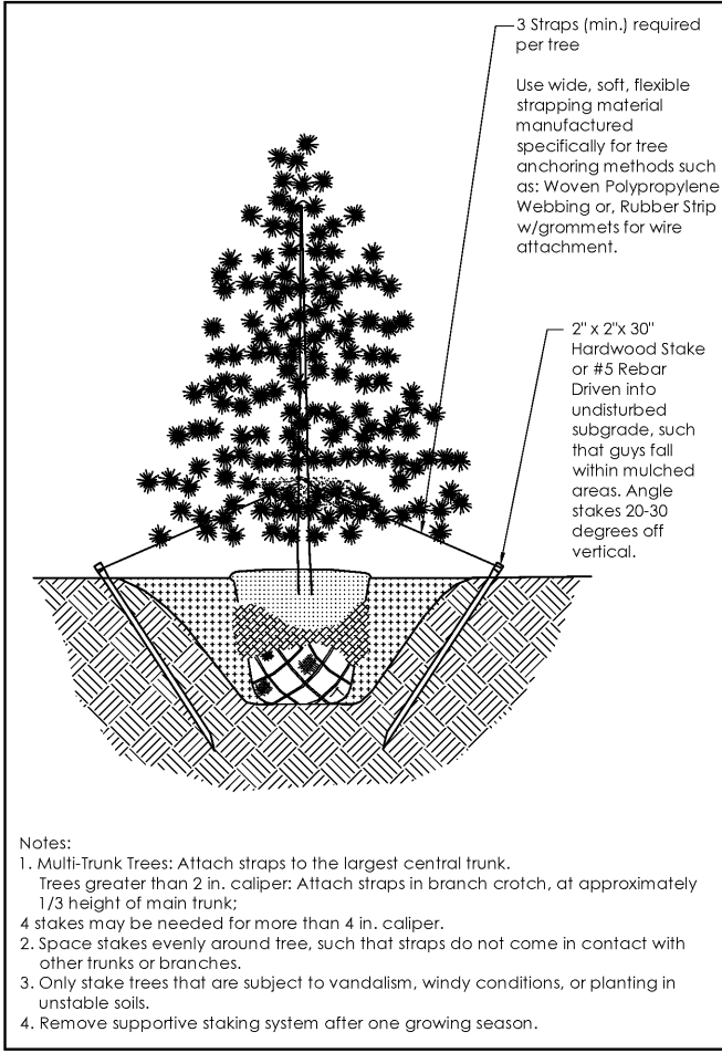
Multi-Trunk & Large Tree Staking Detail (not to scale)
