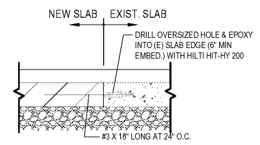
SLAB JOINT DETAIL 2A NTS A-102
