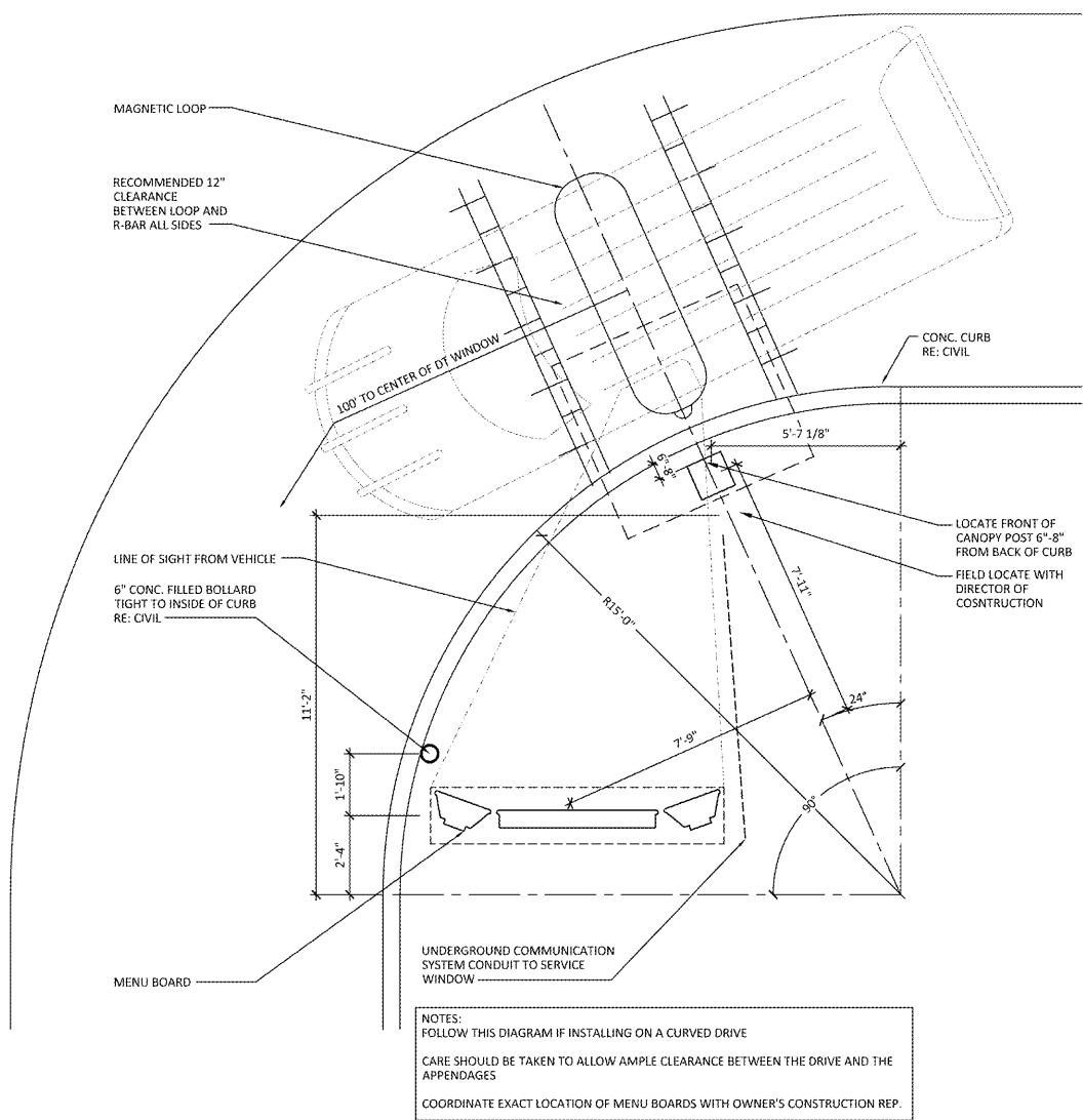
1 DRIVE THRU PLAN - CURVED AS1.3 3/8" = 1'-0"
