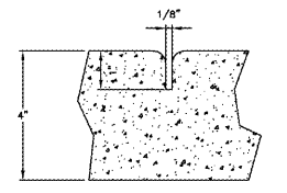
GROOVE JOINT IN SIDEWALK
