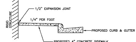
DETAILS SHOWING EXPANSION JOINTS IN CONCRETE SIDEWALK
