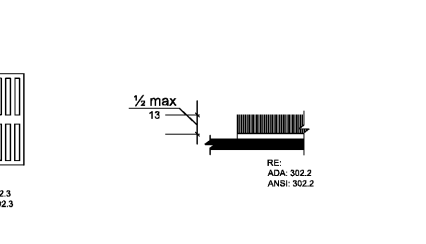
2 FLOOR SURFACE OPENINGS NTS
