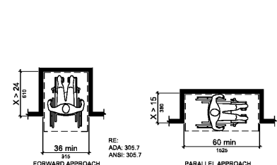
7 ALCOVE CLEARANCES NTS
