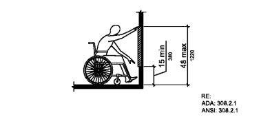
11 UNOBSTRUCTED FORWARD REACH NTS
