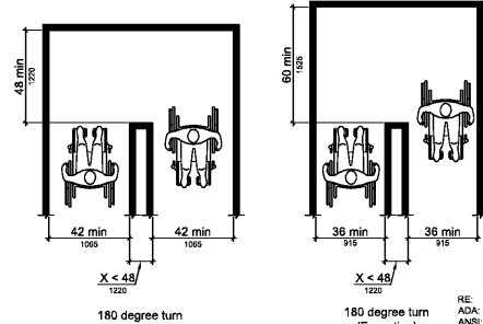
16 CLEAR WIDTH AT 180 DEGREE TURN NTS
