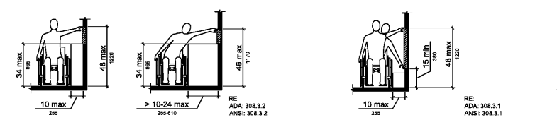
14 OBSTRUCTED HIGH SIDE REACH NTS
