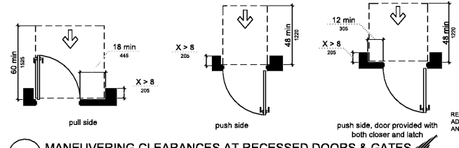
18 MANEUVERING CLEARANCES AT RECESSED DOORS & GATES NTS
