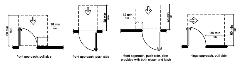
17 MANEUVERING CLEARANCES @ MANUAL SWINGING DOORS & GATES NTS
