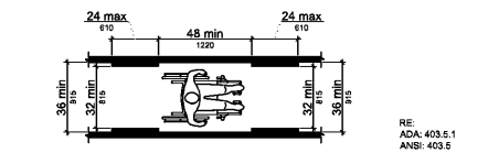
15 CLEAR WIDTH OF ACCESSIBLE ROUTE NTS
