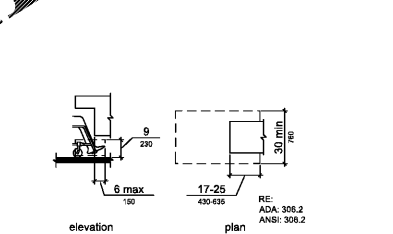
8 TOE CLEARANCES NTS
