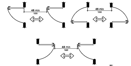
23 DOORS & GATES IN SERIES - DISTANCES NTS
