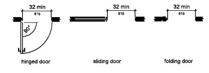
22 CLEAR WIDTH OF DOORWAYS NTS
