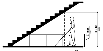
10 VERTICAL CLEARANCE NTS
