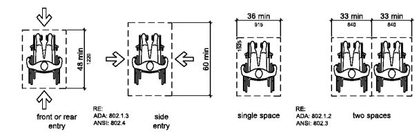
25 SIZE OF WHEELCHAIR SPACES NTS
