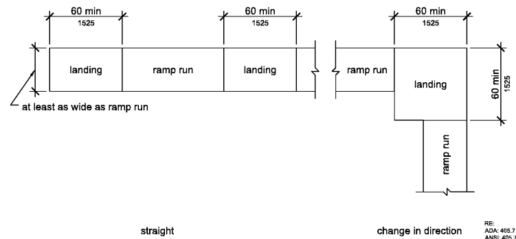
21 RAMP LANDINGS NTS
