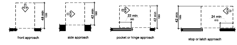
19 MANEUVERING CLEARANCES @ DOORWAYS W/O DOORS, SLIDING DOORS, GATES & FOLDING DOORS NTS
