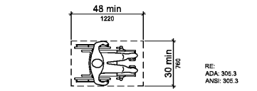
6 CLEAR FLOOR OR GROUND SPACE NTS
