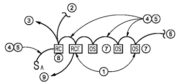
LIGHTING AND RECEPTACLE CONTROL RISER DIAGRAM SCALE: NONE (TYPICAL FOR ALL SPACES UTILIZING ROOM CONTROLLERS)
