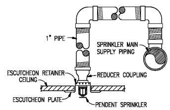
DROP TO PENDENT SPRINKLER HEAD DETAIL SCALE: NONE
