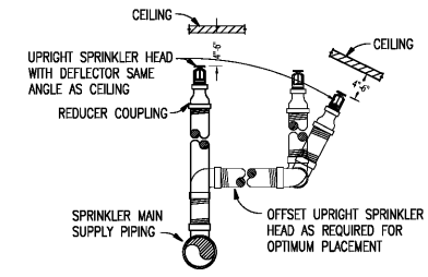
UPRIGHT SPRINKLER HEAD DETAIL SCALE: NONE
