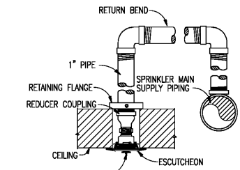
DROP TO INSTITUTIONAL PENDENT SPRINKLER HEAD DETAIL SCALE: NONE
