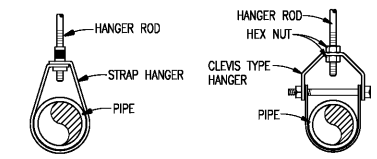
PIPE HANGER DETAIL SCALE: NONE
