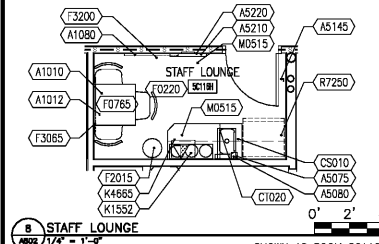
1 STAFF LOUNGE A002 1/4" = 1'-0" SHOWN AS ROOM 5C116H
