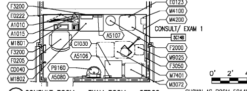
6 CONSULT ROOM - EXAM ROOM - OFDC2 A002 1/4" = 1'-0" SHOWN AS ROOM 5C148 SIM AT 5C102, 5C119 AND 5C154
