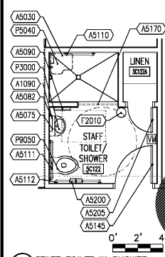
7 STAFF TOILET W SHOWER A002 1/4" = 1'-0" SHOWN AS STAFF TOILET 5C122
