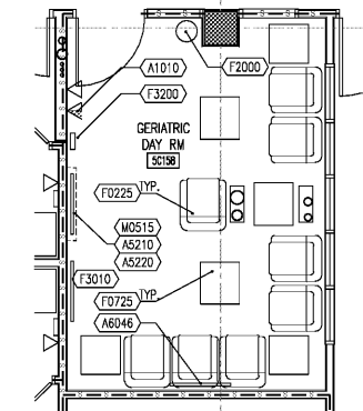
5 DAY ROOM (DAYR1) A002 1/4" = 1'-0" SHOWN AS GERIATRIC DAY ROOM 5C158
