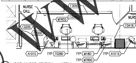
4 LARGE NURSE STATION - NSTA1 A002 1/4" = 1'-0" SHOWN AS ROOM 5C120 SIM AND MIRRORRED AT 5C157
