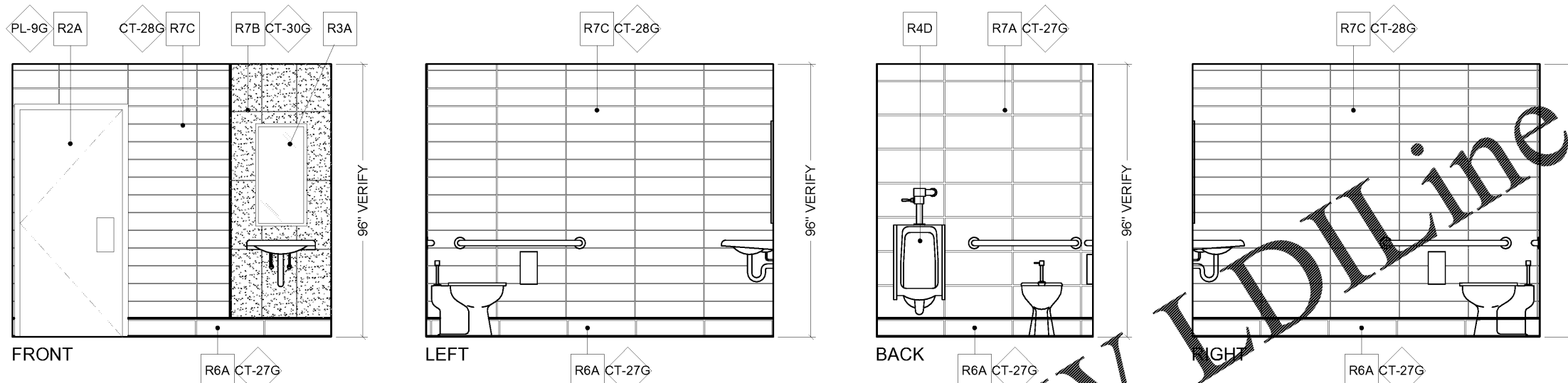
TYPICAL RESTROOM FINISH ELEVATIONS RE : WALL FINISH PLAN
