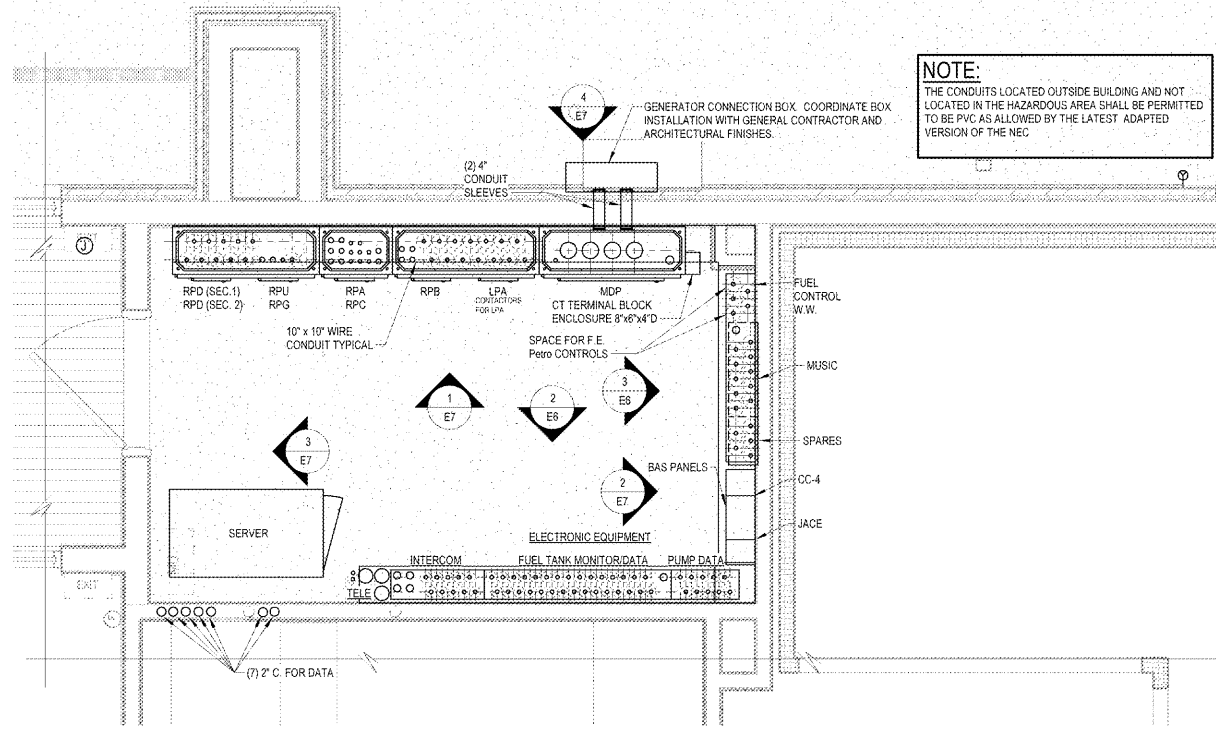
1 ELECTRICAL ROOM LAYOUT PLAN E6 1/2" = 1'-0"
