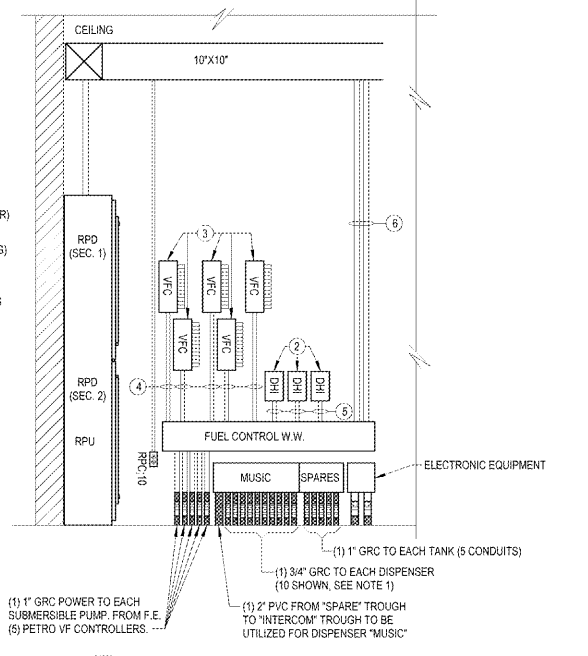
3 ELECTRICAL ROOM SPARE CONDUITS ELEVATION E6 1/2" = 1'-0"
