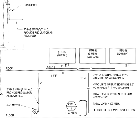
2 GAS RISER NOT TO SCALE
