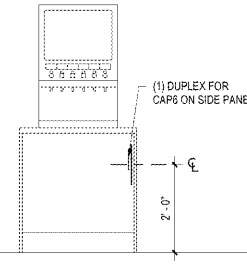
CAPPUCCINO ELEVATION VIEW B29.1
