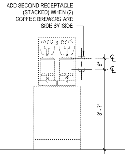
COFFEE BREWER ELEVATION VIEW B26.2
