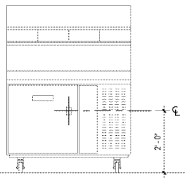
REFRIGERATED FOOD PREP UNIT ELEVATION VIEW
