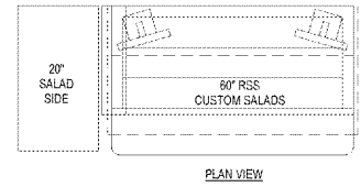
PLAN VIEW
