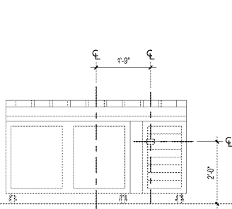
REFRIGERATED SANDWICH STATION ELEVATION VIEW
