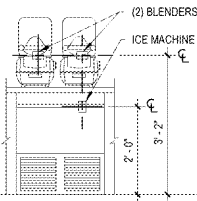
BLENDER W/ ICE MACHINE BELOW ELEVATION VIEW
