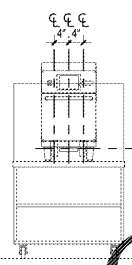
TOASTER ON FRONT LINE W/ ROLLING CABINET ELEVATION VIEW
