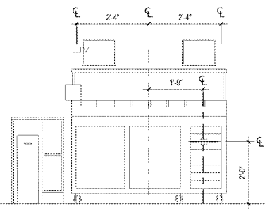
BUILT TO ORDER - 60" RSS ELEVATION VIEW
