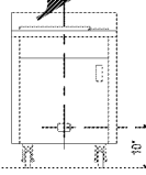
RE THERMALIZER ELEVATION VIEW
