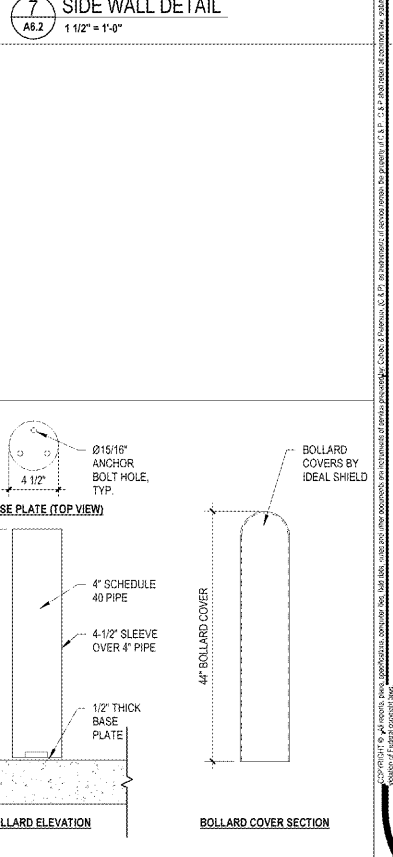
8 GENERATOR BOX BOLLARD SECTION A6.2 1 1/2" = 1'-0"
