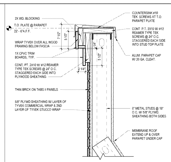
2 PARAPET DETAIL A6.2 1 1/2" = 1'-0"
