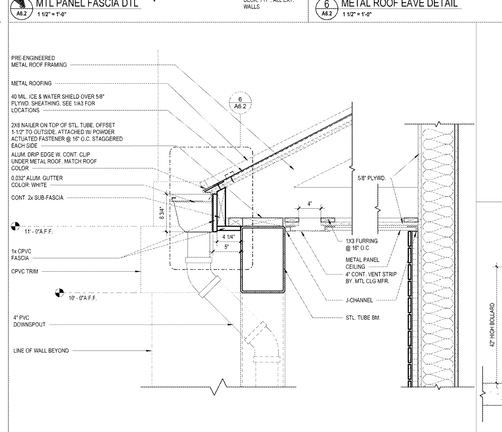
4 PORCH EAVE DETAIL A6.2 1 1/2" = 1'-0"
