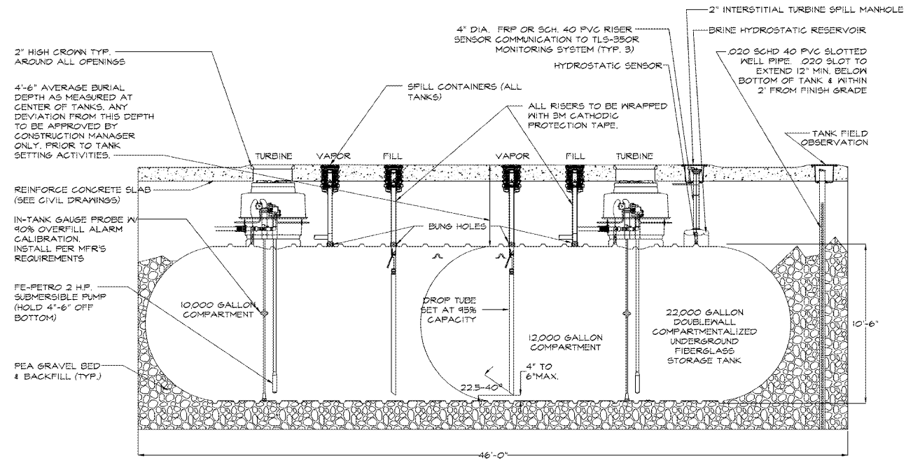
A TYPICAL COMPARTMENTALIZED TANK SECTION G-2 SCALE: 1/4"=1'-0"
