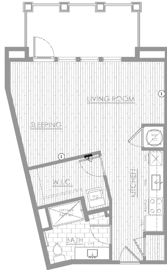
2 UNIT S2 14'4" x 12'
