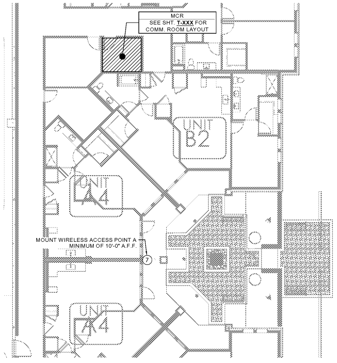
2 01-EAST COURTYARD SCALE: 3/32"=1'-0"
