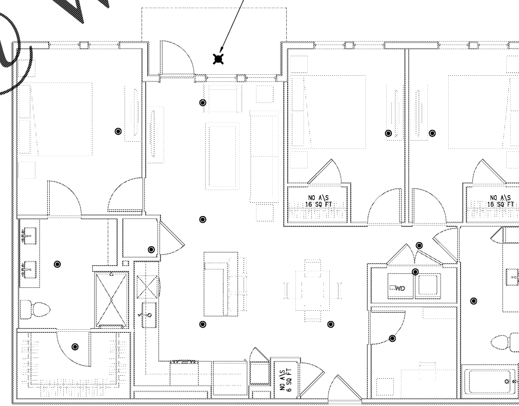
2 UNIT C1-A - FIRE PROTECTION PLAN SCALE: 1/4"=1'-0"
