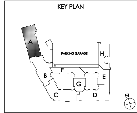
1 PARTIAL BUILDING PLAN A - (00) BASEMENT - FIRE PROTECTION PLAN SCALE: 1/8" = 1'-0" 18026-F-BLDG
