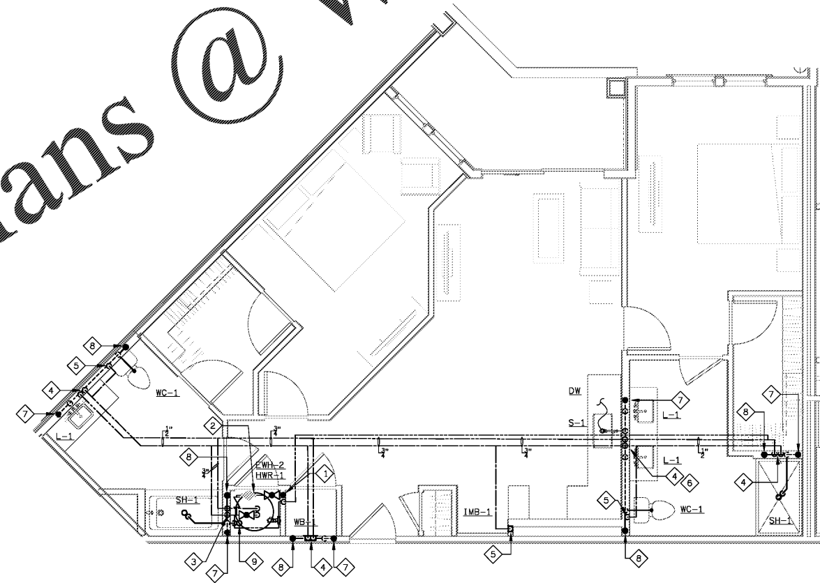
2 UNIT B6 - PLUMBING PLAN SCALE: 1/4"=1'-0" 18025-P-UNIT
