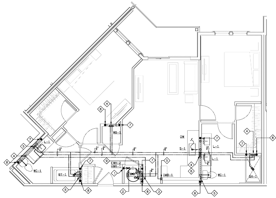
2 UNIT B2 - PLUMBING PLAN SCALE: 1/4"=1'-0" 880225-P-UNIT
