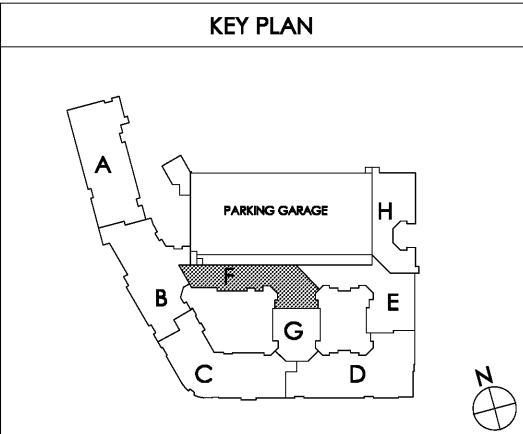
1 PARTIAL BUILDING PLAN F - (05) ROOF - PLUMBING PLAN SCALE: 1/8" = 1'-0" 18025-P-BLDG
