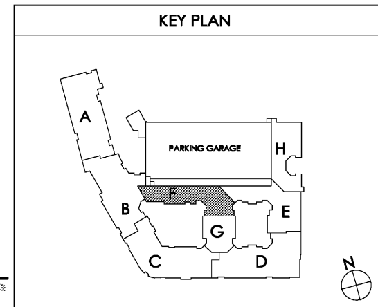
1 PARTIAL BUILDING PLAN F - (02) SECOND FLOOR - PLUMBING PLAN SCALE: 1/8" = 1'-0" 18025-P-BLDG
