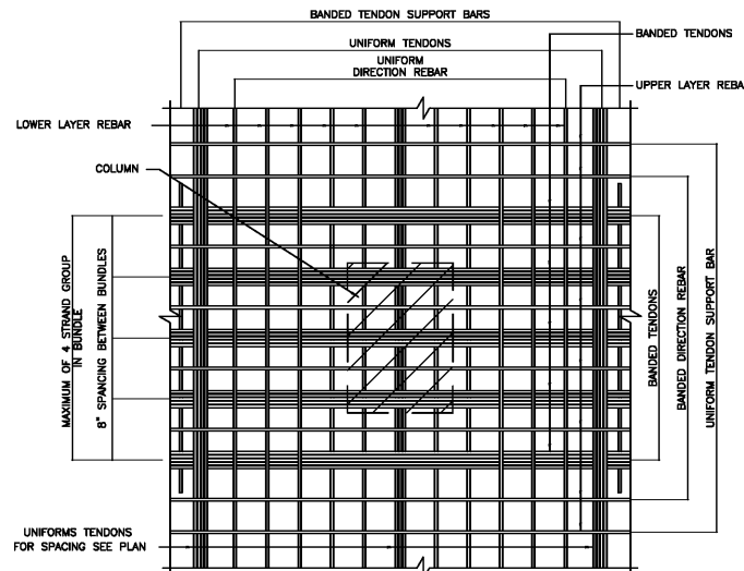
41 PLAN VIEW AT COLUMN UNIFORM TENDONS AT COLUMN CENTERLINE-TIED UNDER BANDED TENDONS N.T.S.
