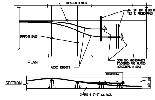
39 PLACEMENT OF ADDED TENDON IN CORROSIVE ENVIRONMENT N.T.S.
