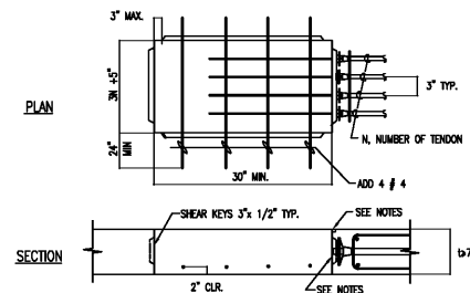
50 STRESSING BLOCKOUT IN CORROSIVE ENVIRONMENT N.T.S.
