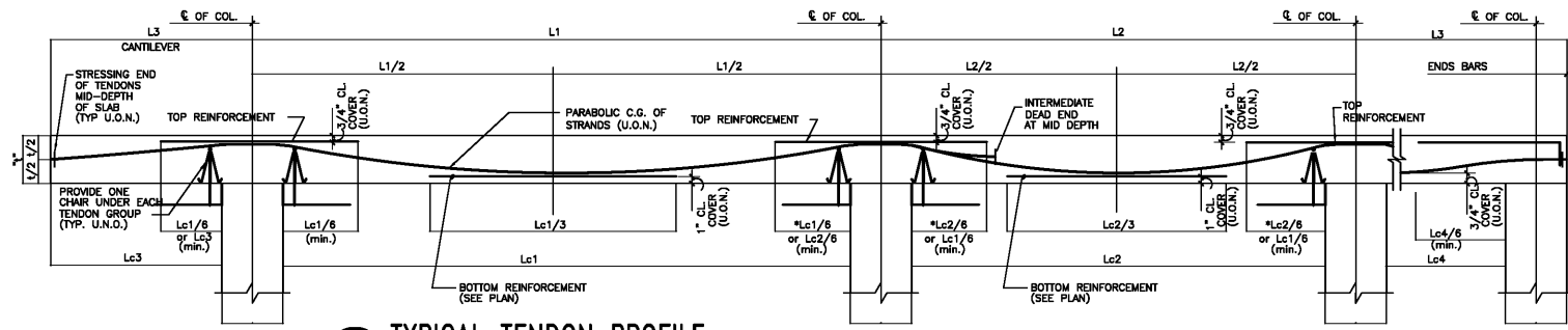
38 TYPICAL TENDON PROFILE NOTE: 1. WHEN THE LENGTH OF THE TOP REINFORCEMENT IS NOT INDICATED ON PLAN TAKE TOTAL LENGTH, AS INDICATED IN DETAIL # N.T.S.
