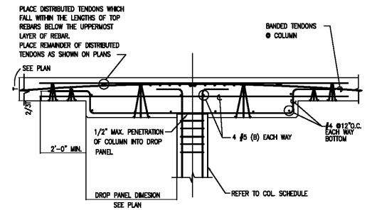
48 TYPICAL DROP PANEL SECTION N.T.S.
