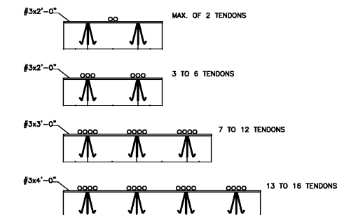
52 TYPICAL TENDON DISTRIBUTION AND SUPPORT DETAIL N.T.S.
