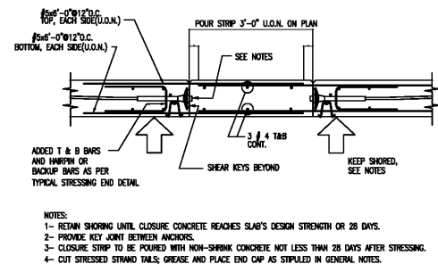
47 POUR STRIP IN SLAB FOR CORROSIVE ENVIRONMENT N.T.S.
