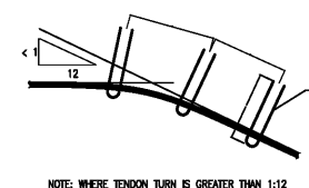
51 TENDON PLACEMENT FOR TURNS >1:12 N.T.S.
