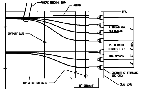
42 FLARING OF BANDED TENDONS AT SLAB EDGE IN CORROSIVE ENVIRONMENT N.T.S.
