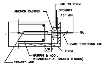
45 STRESSING END ANCHOR IN CORROSIVE ENVIRONMENT N.T.S.
