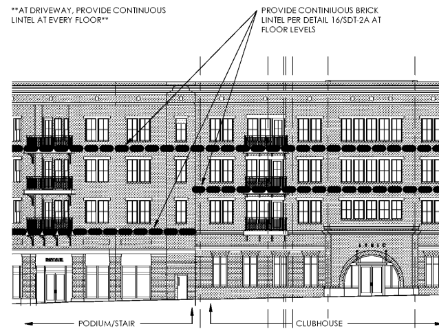
1 CONTINUOUS LINTEL LOCATIONS DIAGRAM SCALE: 1/16" = 1'-0"
