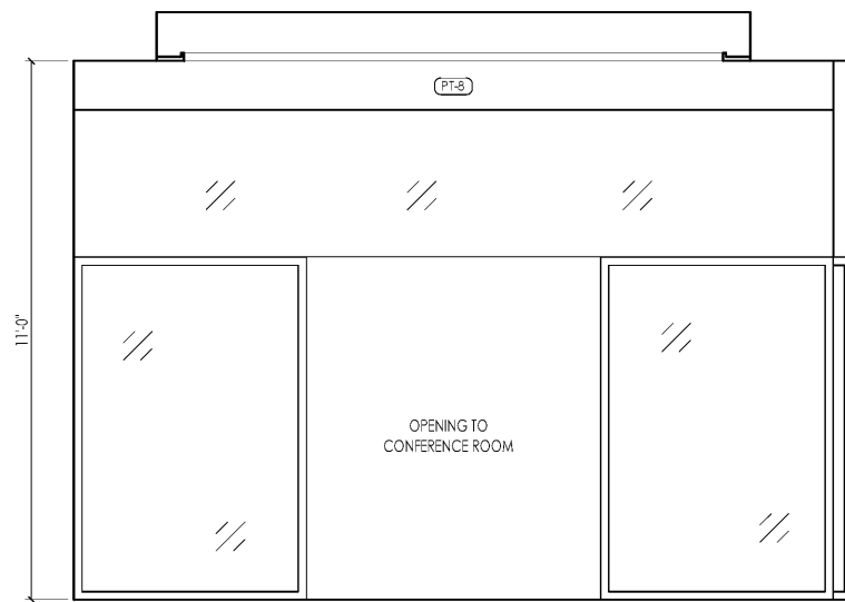
1 ELEVATION @ CONFERENCE ROOM ID8.02 SCALE: 1/2" = 1'-0"
