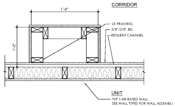
1 CORRIDOR DETAIL CORRIDOR COLUMN DETAIL SCALE: 1 1/2" = 1'-0"
