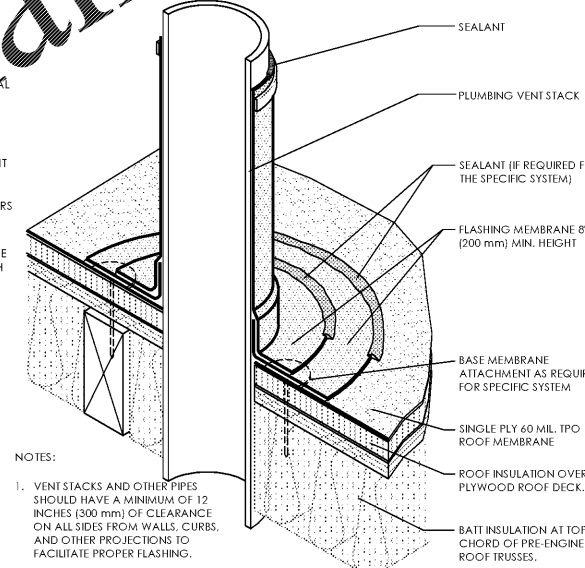
5 PLUMBING VENT
