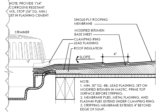
6 ROOF DRAIN DETAIL
