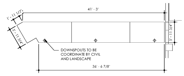
2 AWNING #3 ENLARGED SCALE: 1/8" = 1'-0"
