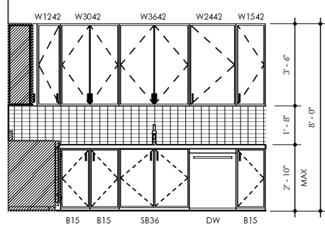
13 KITCHEN UNIT C1-A SCALE: 3/8" = 1'-0"
