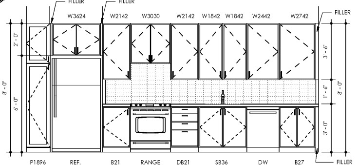
8 KITCHEN UNIT B5-A SCALE: 3/8" = 1'-0"
