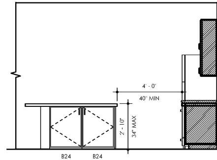
11 KITCHEN UNIT C1-A SCALE: 3/8" = 1'-0"
