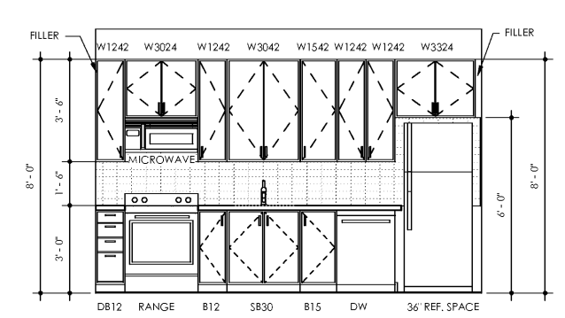
1 KITCHEN UNITS S1 SCALE: 3/8" = 1'-0"
