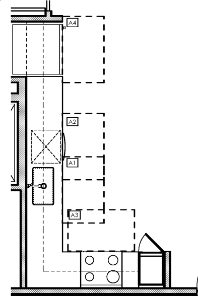
1 KITCHEN UNIT B3 SCALE: 3/8" = 1'-0"
