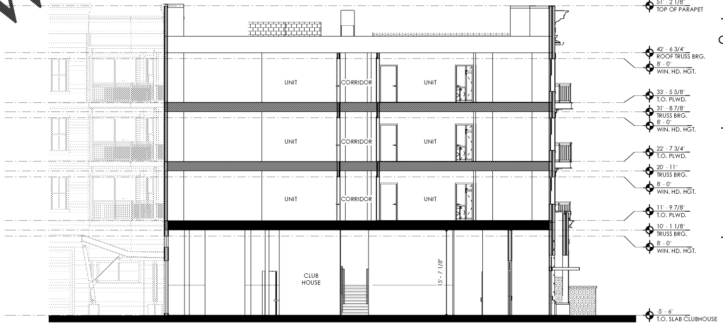
1 BUILDING TWO - SECTION (1) SCALE: 1/8" = 1'-0"
