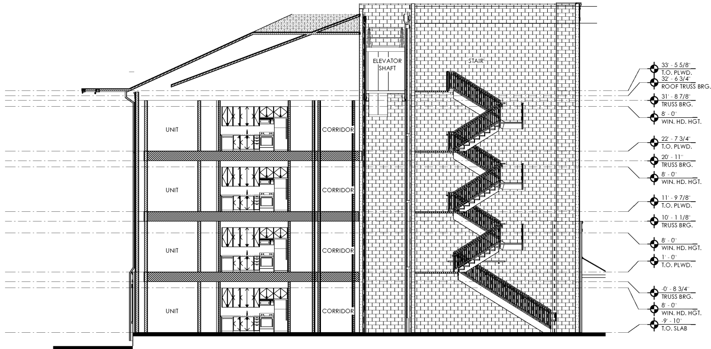
4 BUILDING TWO - SECTION (4) SCALE: 1/8" = 1'-0"
