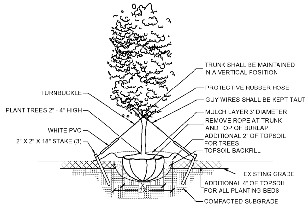
TYPICAL TREE PLANTING CROSS SECTION - N.T.S.
