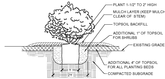
TYPICAL SHRUB PLANTING CROSS SECTION - N.T.S.
